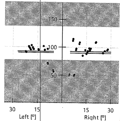
Accuracy [%]
