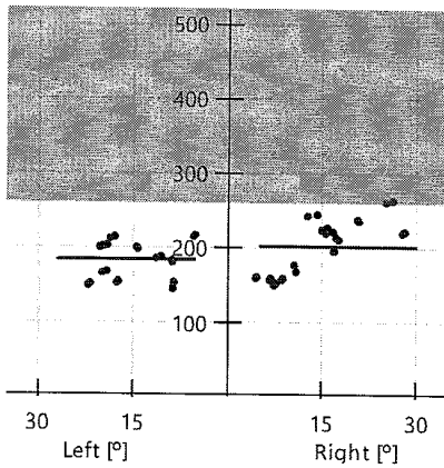
Latency [ms]
